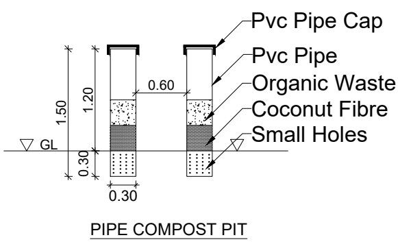
PIPE COMPOST PIT
