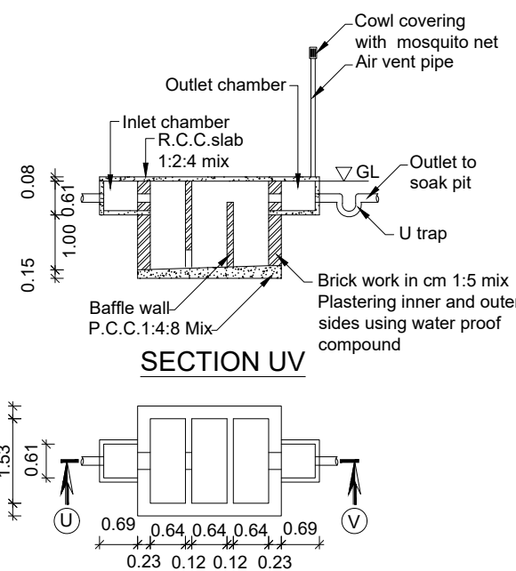
SECTION UV
