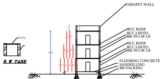
SECTION ON AJ
