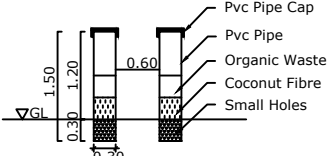
PIPE COMPOST PIT
