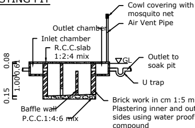
SECTION UV
