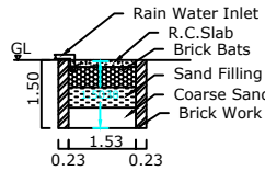
RAIN WATER HARVESTING PIT
