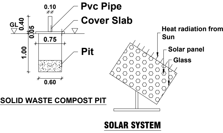
SOLAR SYSTEM
