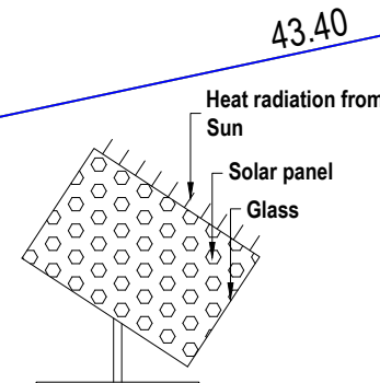
SOLAR SYSTEM
