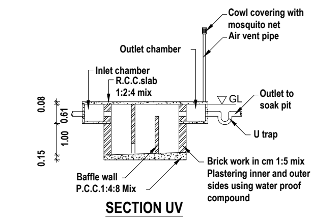
SECTION UV
