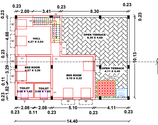
PRO. FIRST FLOOR
