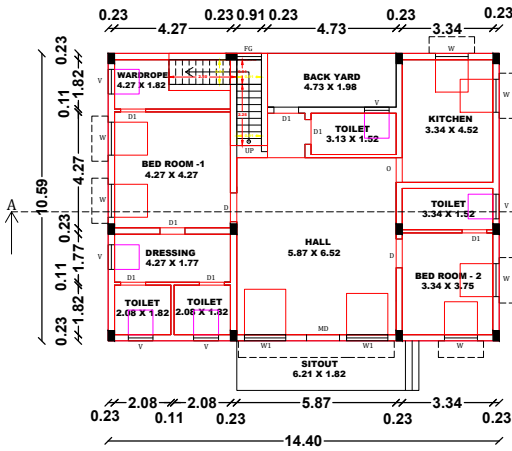
PRO. GROUND FLOOR
