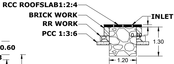
RAIN WATER HARVEST TRENCH
