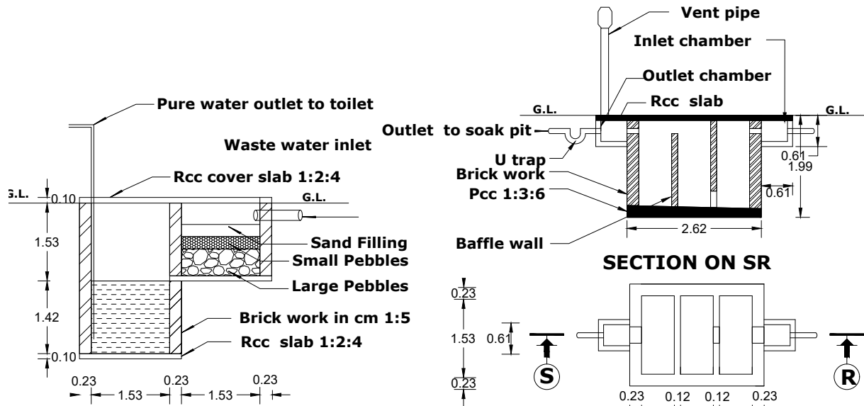
WASTE WATER RECYCLING SYSTEM
