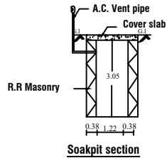
Soakpit section
