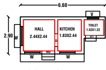
GROUND FLOOR PLAN SCALE 1:100 ALL DIMS ARE IN METRE
