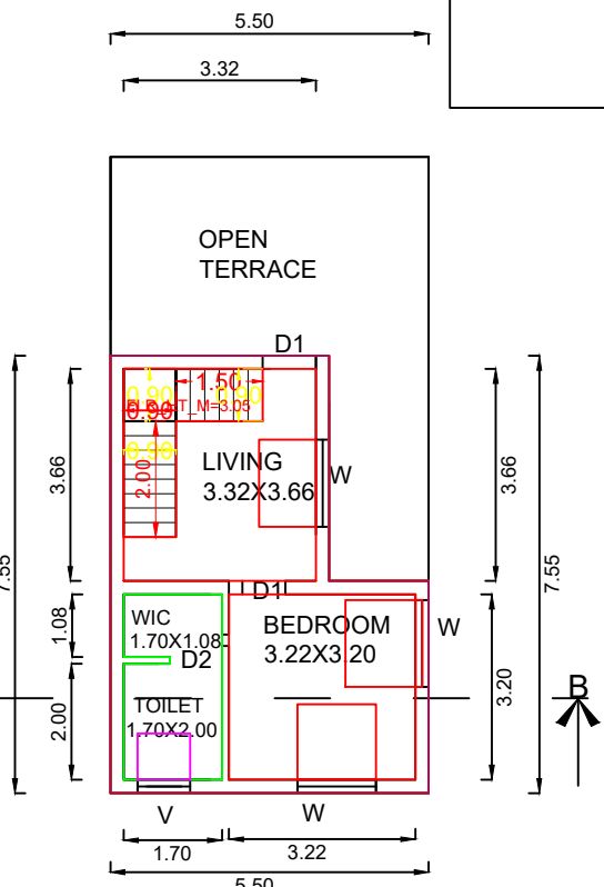
FF PLAN
