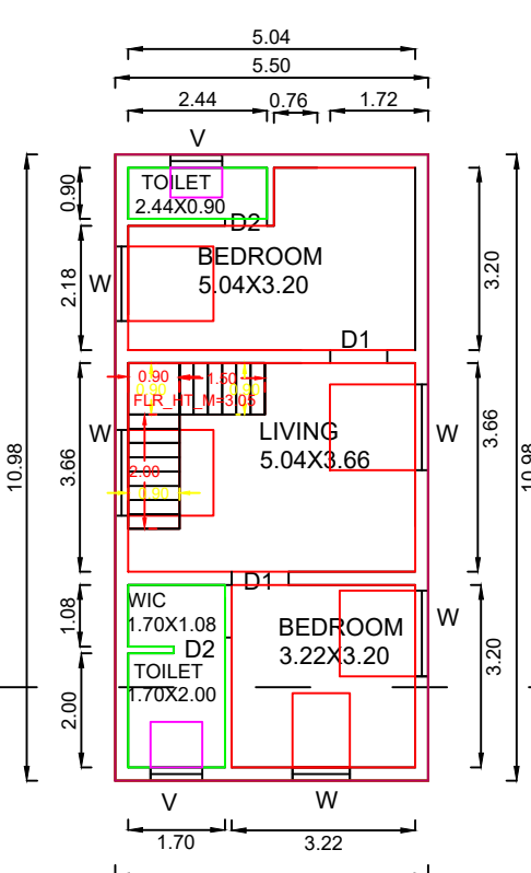
FF PLAN
