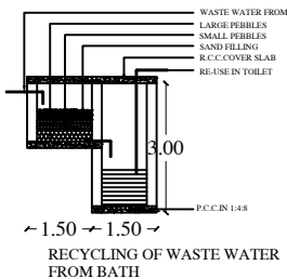
RECYCLING OF WASTE WATER FROM BATH
