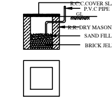
RAIN WATER HARVEST ARRANGEMENTS
