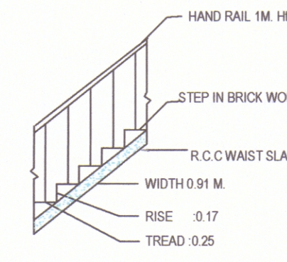
STAIR DETAIL
