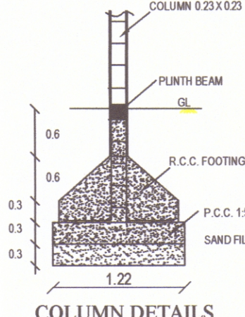
COLUMN DETAILS
