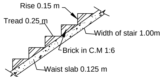
STAIR DETAILS
