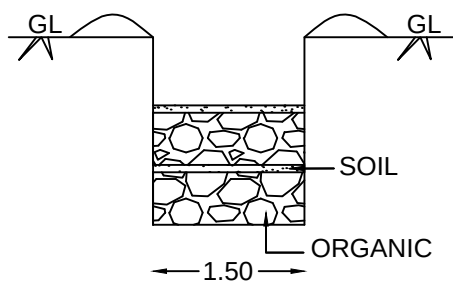
COMPOST PIT
