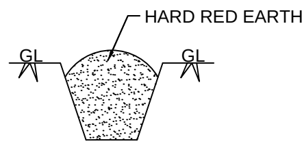
TRIAL PIT SECTION
