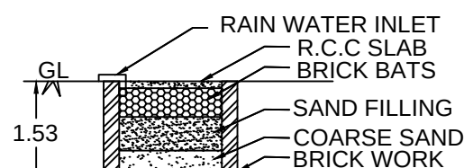
RAIN WATER HARVESTING
