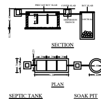
SEPTIC TANK
