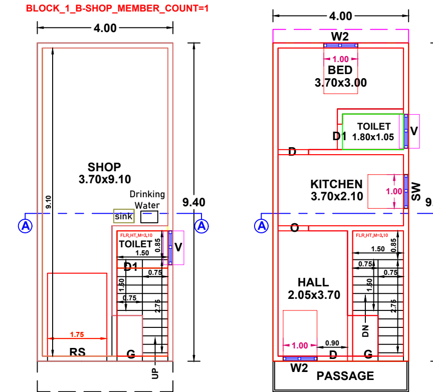
GROUND FLOOR PLAN FIRST FLOOR PLAN
