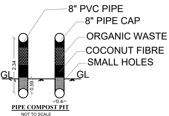
PIPE COMPOST PIT NOT TO SCALE
