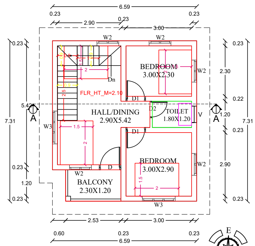
FIRST FLOOR PLAN AREA =47.33 Sq.M (509.27Sq.ft)
