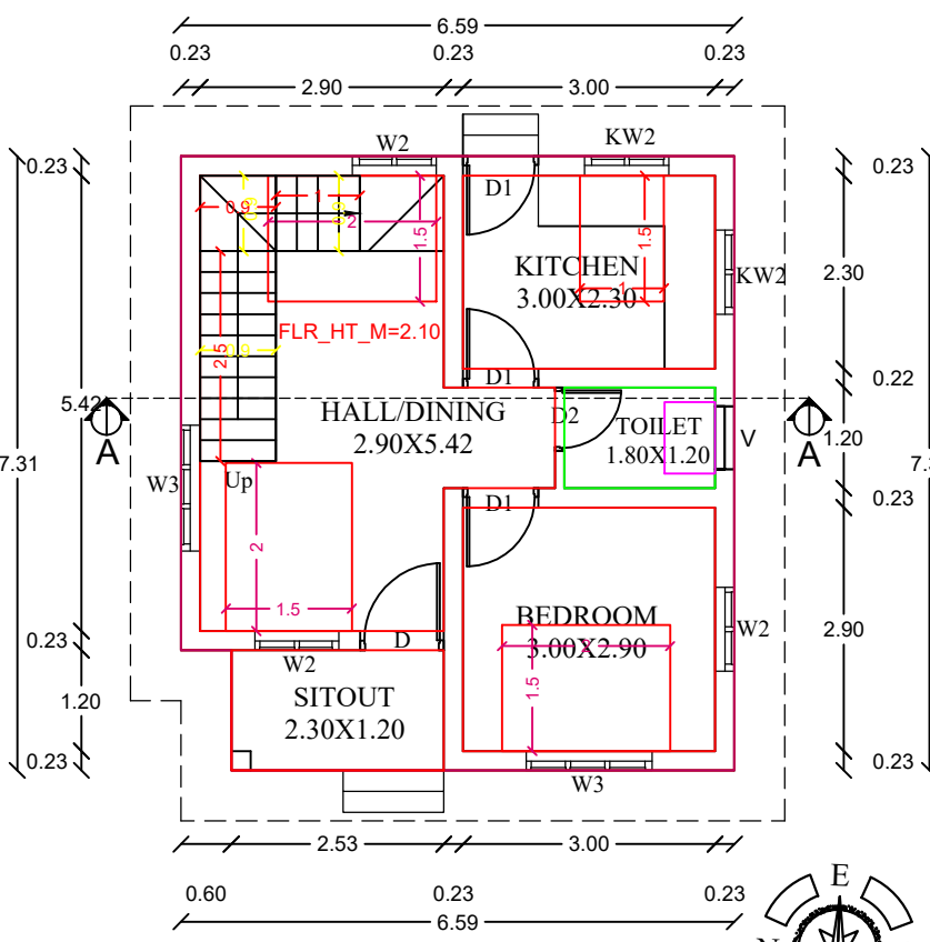
GROUND FLOOR PLAN AREA =47.33 Sq.M (509.27Sq.ft)
