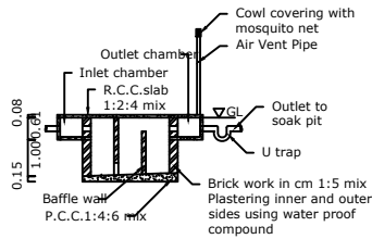
SECTION UV
