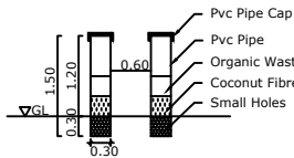
PIPE COMPOST PIT
