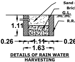
DETAILS OF RAIN WATER HARVESTING
