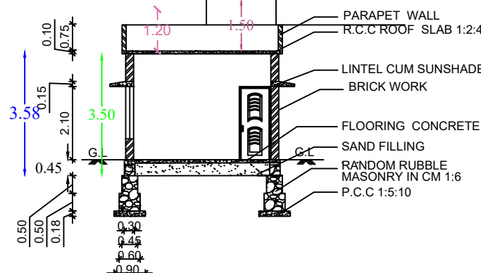
SECTION ON-CD
