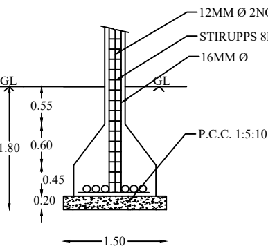
COLUMN DETAILS (SIZE 0.23X0.30)
