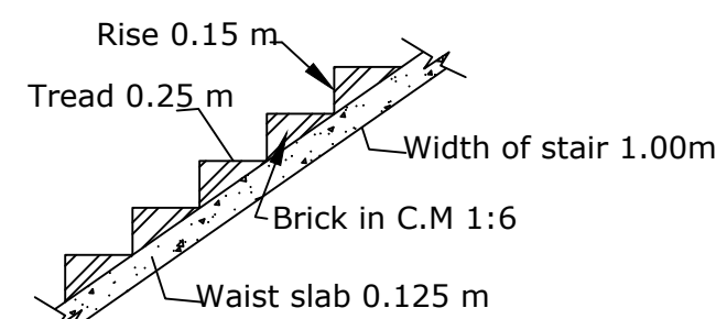
STAIR DETAILS
