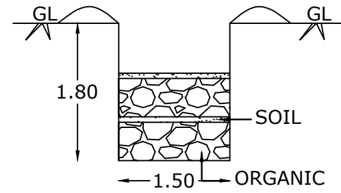
COMPOST PIT
