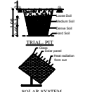
SOLAR SYSTEM
