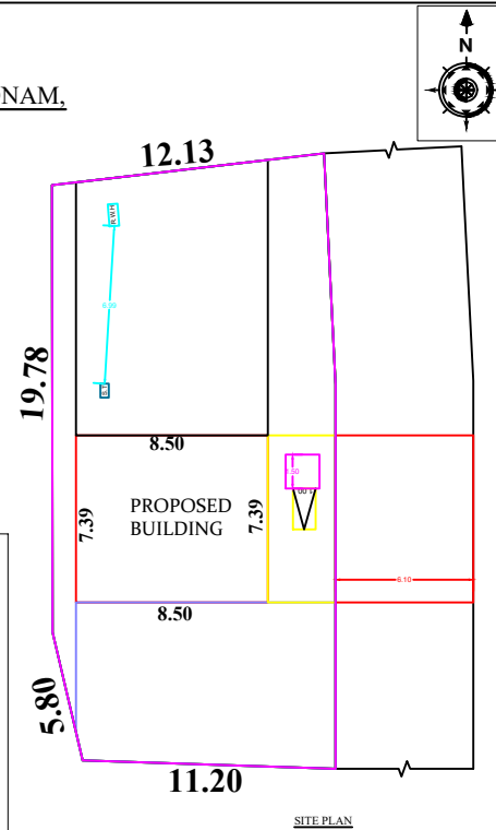
SITE PLAN
