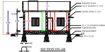
SECTION ON-AB
