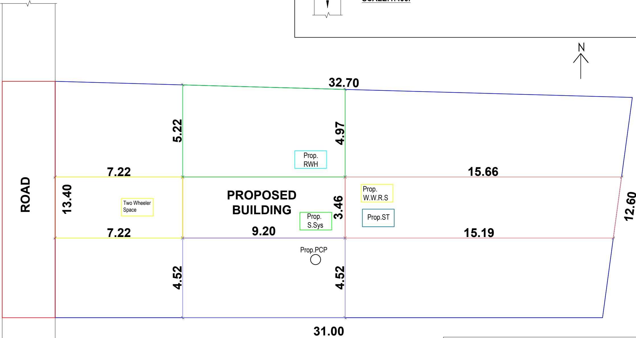
KEY PLAN SCALE:1:400.
