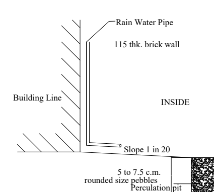
PERCOLATION PIT
