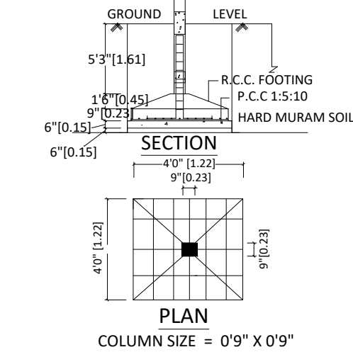
FOUNDATION DETAILS
