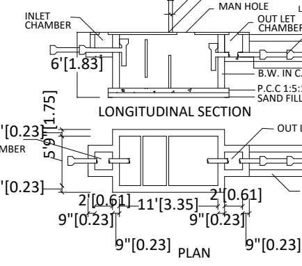
SEPTIC TANK:
