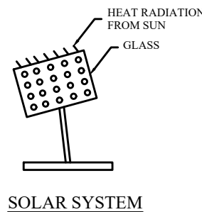
SOLAR SYSTEM
