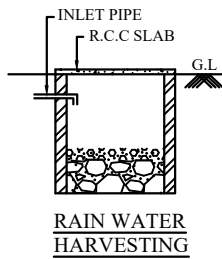
RAIN WATER HARVESTING
