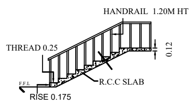
STAIRCASE DETAILS
