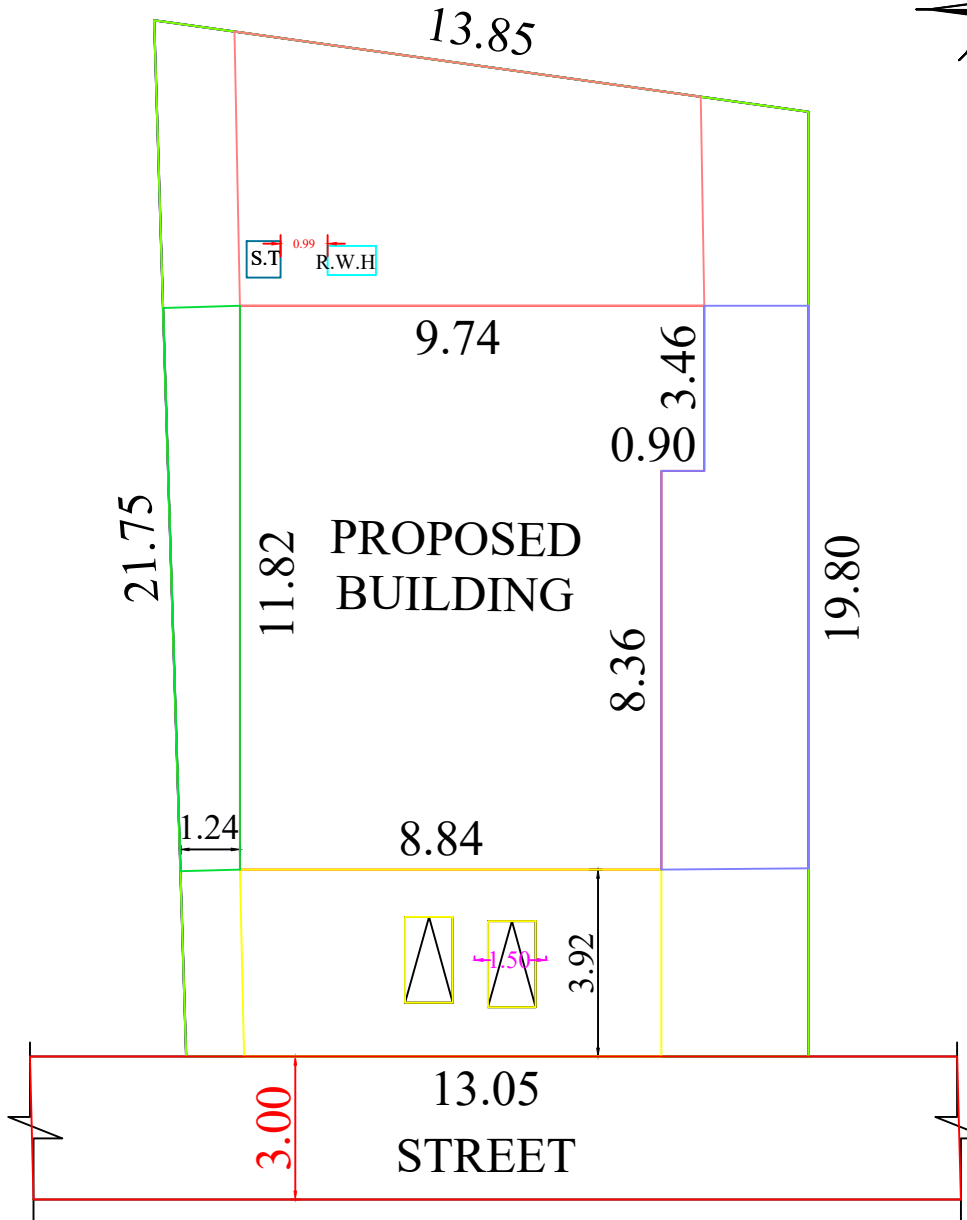
SITE PLAN
