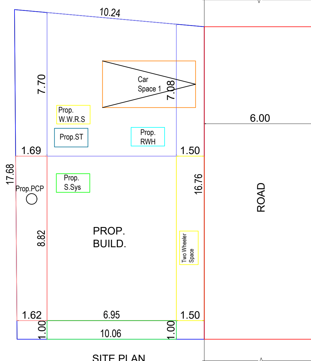
SITE PLAN
