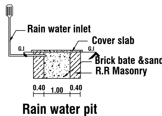
Rain water pit
