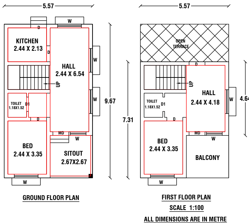
ALL DIMENSIONS ARE IN METRE
