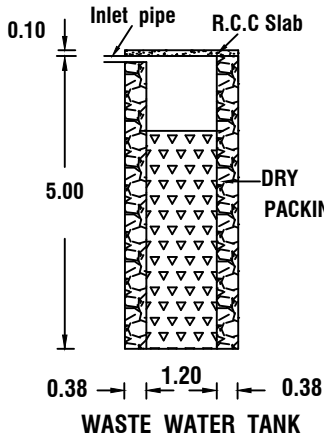
WASTE WATER TANK
