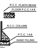
TYP.DETAILS OF COLUMNS
