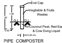
PIPE COMPOSTER
