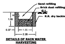
DETAILS OF RAIN WATER HARVESTING
