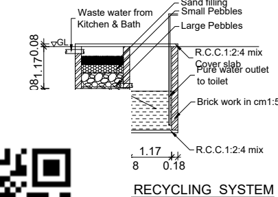
RECYCLING SYSTEM
