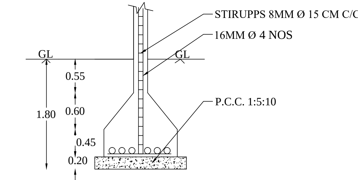
COLUMN DETAILS (SIZE 0.23X0.23)
