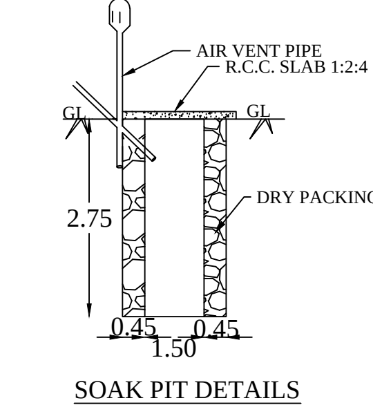
SOAK PIT DETAILS
