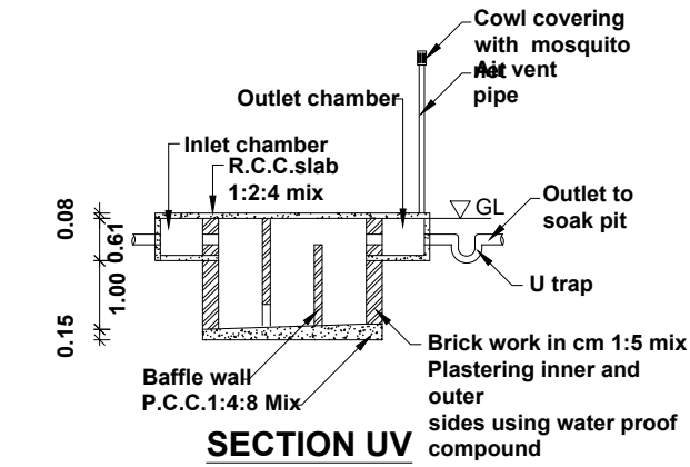
SECTION UV
