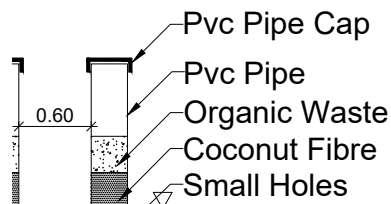
COMPOST PIT
