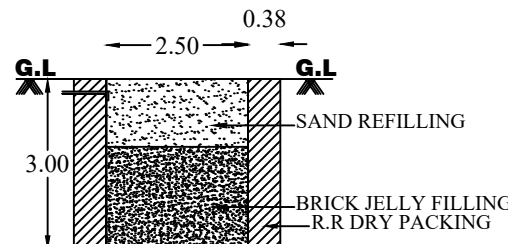
RAINWATER HARVESTING
