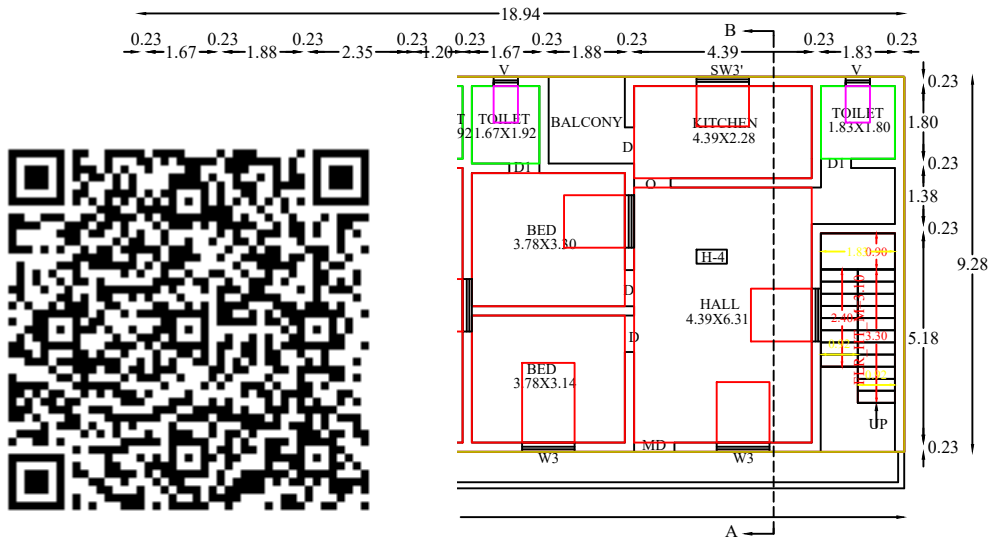
2 FLOOR PLAN
