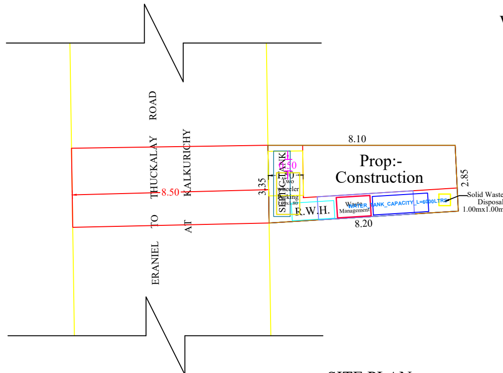
SITE PLAN
