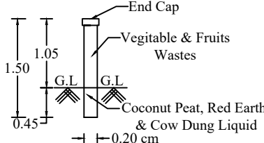
PIPE COMPOSTER
