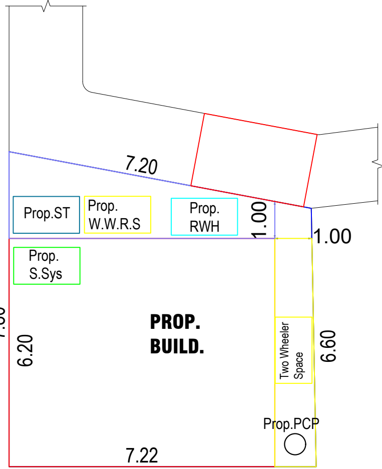
SITE PLAN
