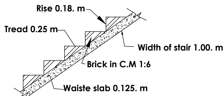
STAIR DETAILS
