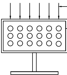
SOLAR SYSTEM
