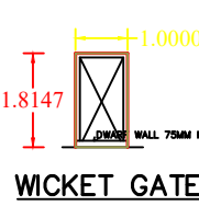
WICKET GATE
