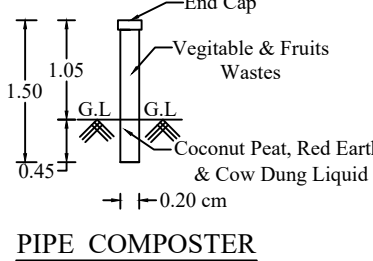
PIPE COMPOSTER
