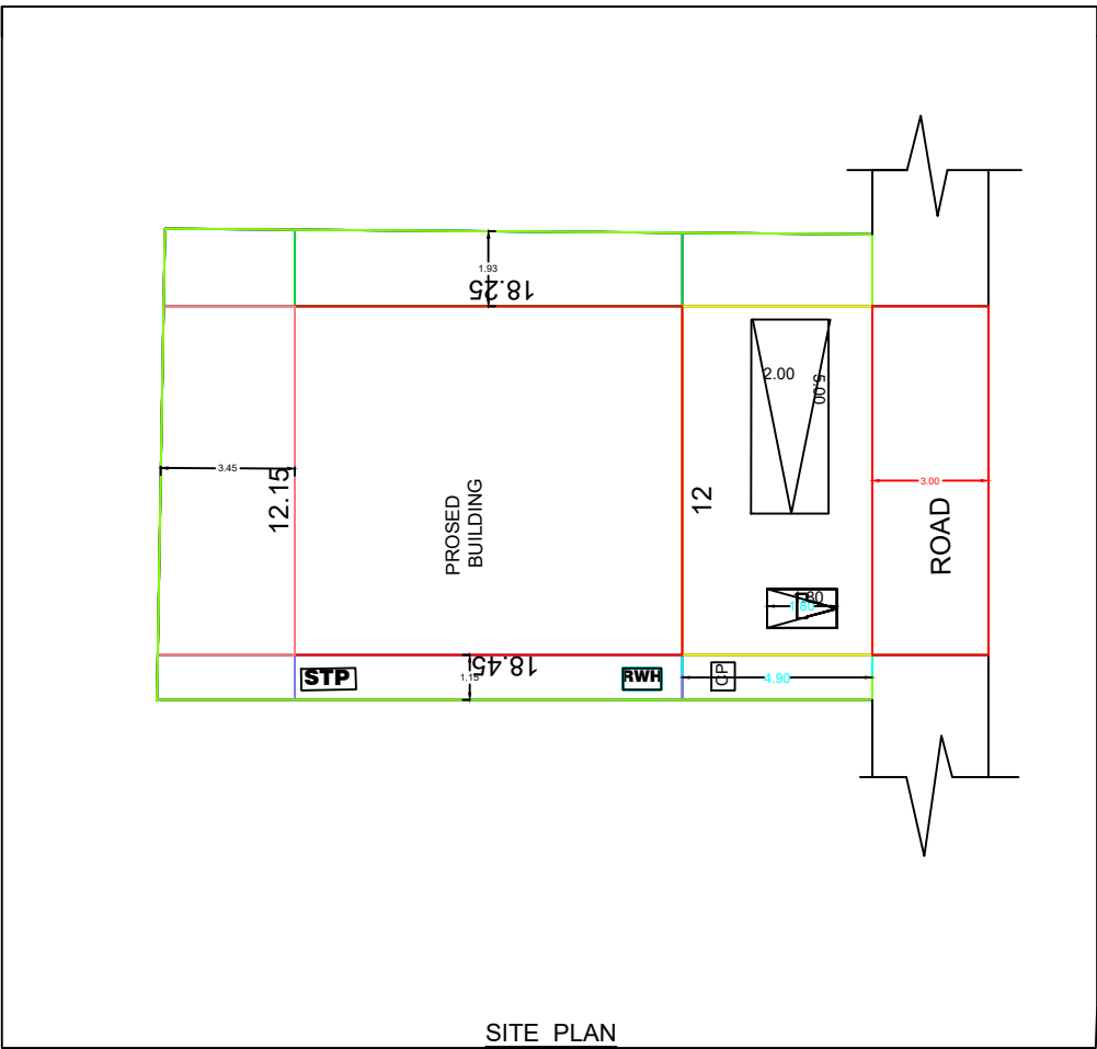
SITE PLAN
