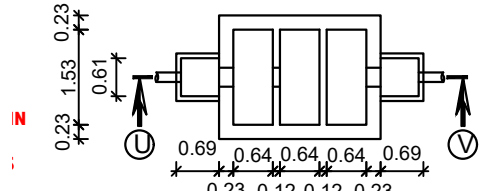
SEPTIC TANK PLAN
