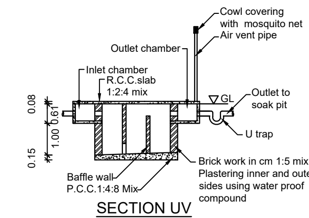
SECTION UV
