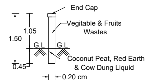
PIPE COMPOSTER
