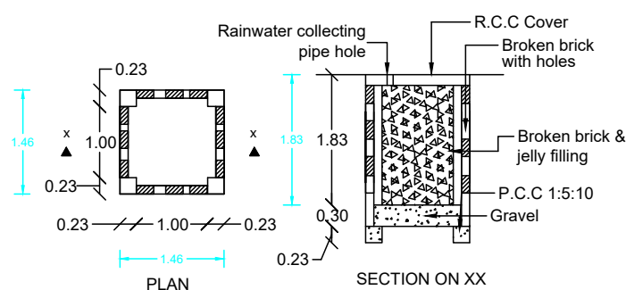
RAIN WATER HARVEST WELL
