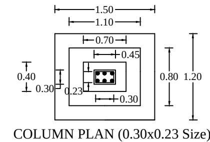
COLUMN PLAN (0.30x0.23 Size)
