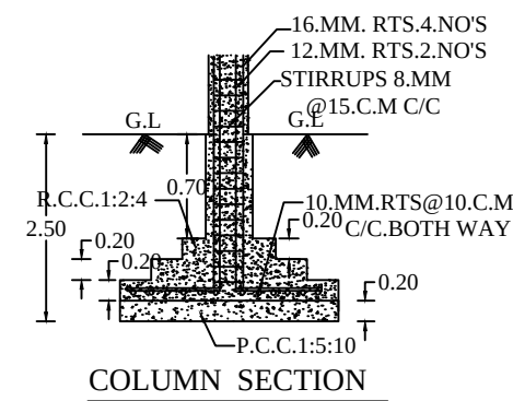
COLUMN SECTION
