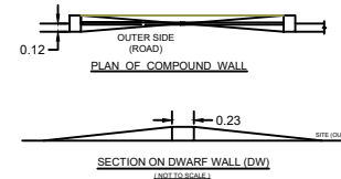
PLAN OF COMPOUND WALL
