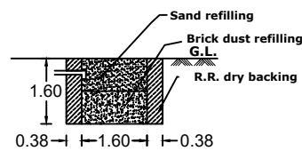
DETAILS OF RAIN WATER HARVESTING
