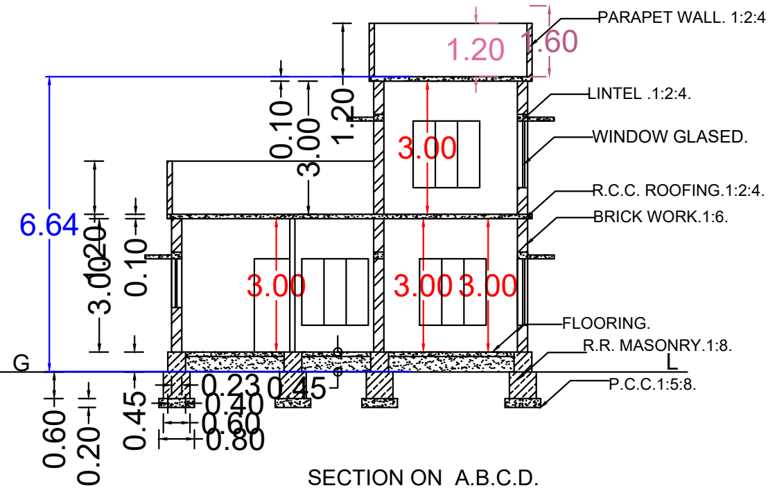
SECTION ON A.B.C.D.
