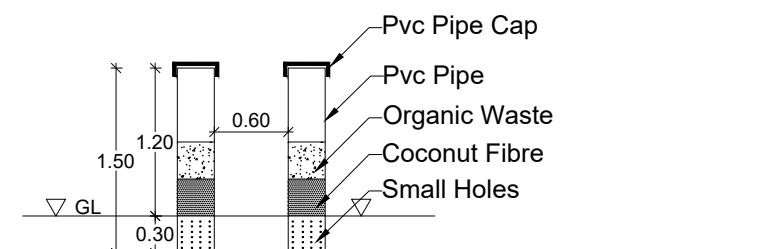
PIPE COMPOST PIT
