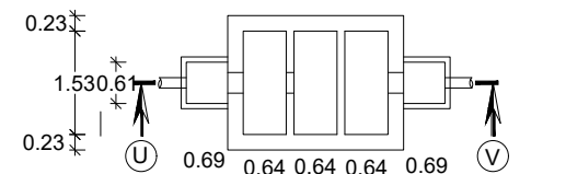
SECTION UV
