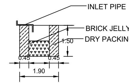
RAINWATER HARVESTING
