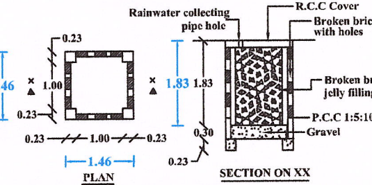
RAIN WATER HARVEST WELL
