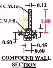
COMPOUND WALL SECTION
