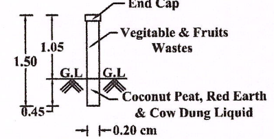
PIPE COMPOSTER
