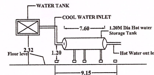
SOLAR WATER HEATING SYSTEM (S.W.H.S.DETAILS)
