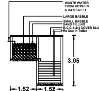
RECYCLING OF WASTE WATER FROM BATHROOM & KITCHEN
