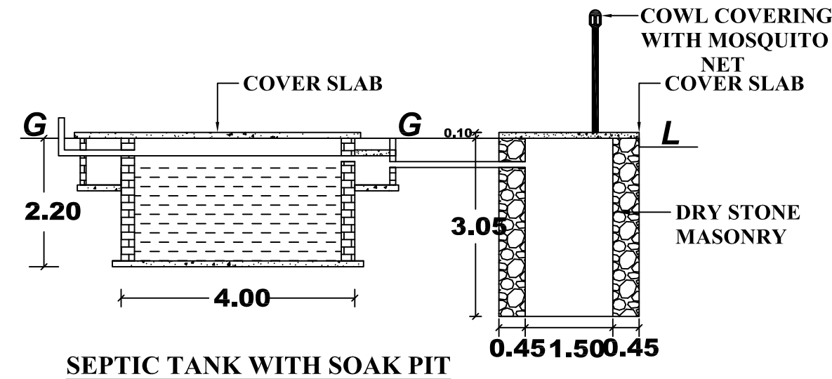
SEPTIC TANK WITH SOAK PIT
